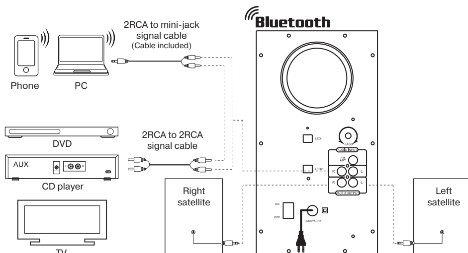
Fig. 5. Connection diagram
