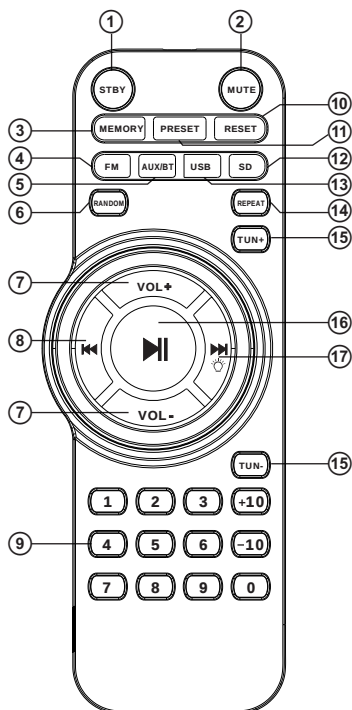
Fig. 4. Remote control
